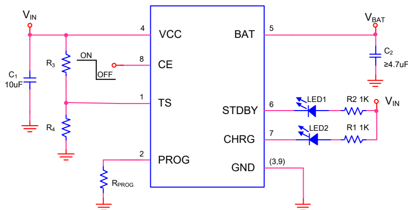
Figure 1. HE4066H Typical Application Circuit
