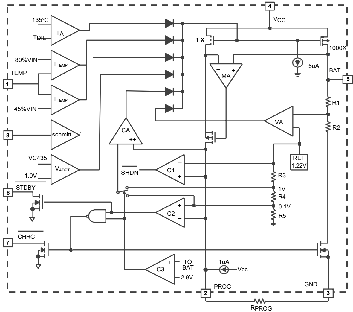
Figure 2.HE4066H Block Diagram
