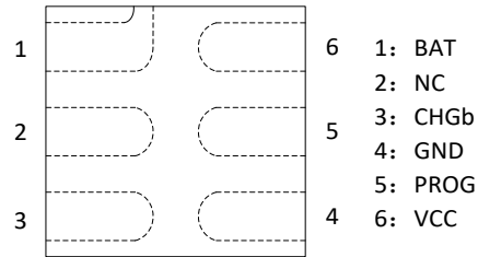
HE4051Y (Top view) TDFN1X1-6L
