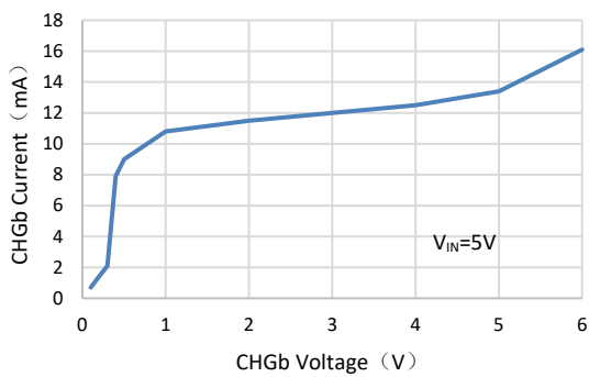
CHGb Current vs. CHGb Voltage
