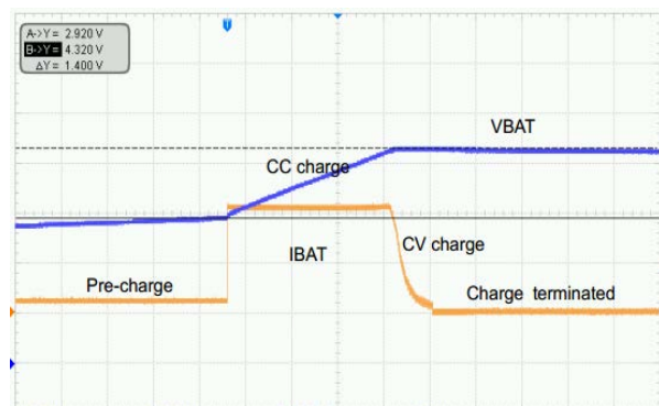
Charge Curve
