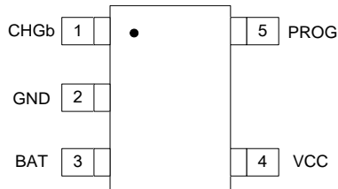
HE4051N (Top view) SOT23-5L
